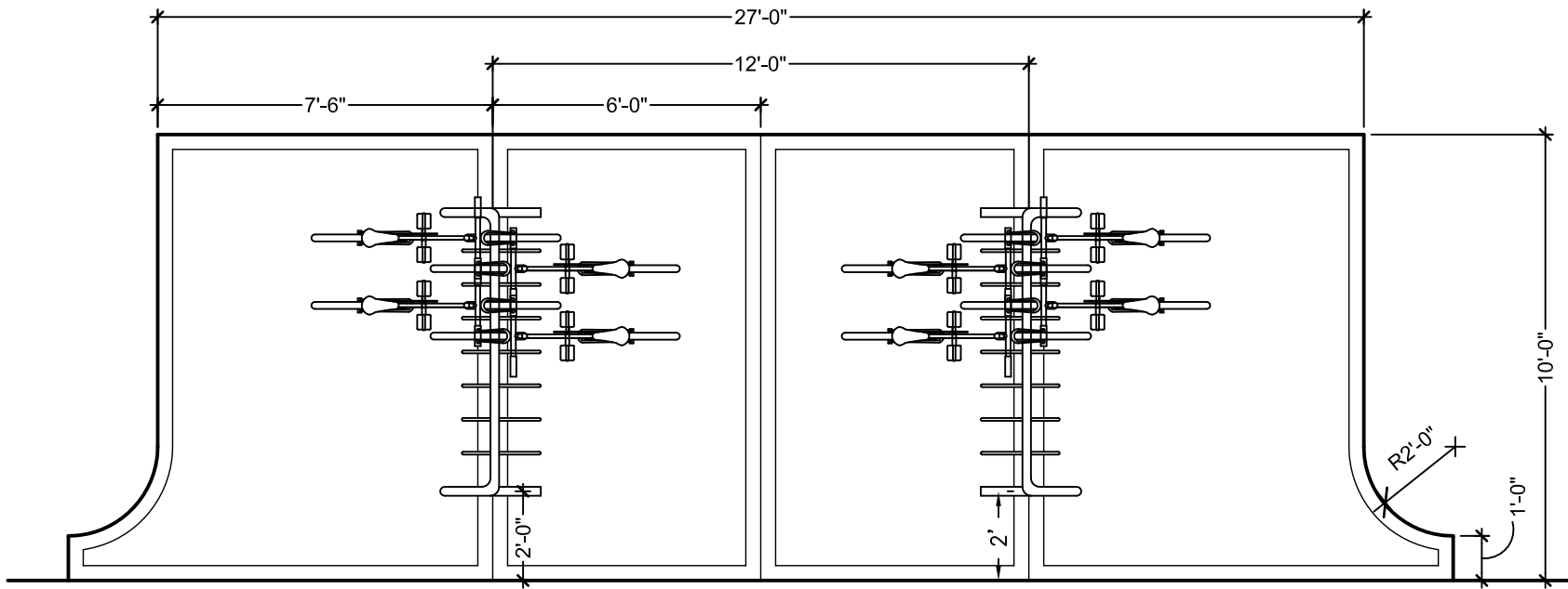
TYPICAL BICYCLE RACK LAYOUT SCALE: 1/4"=1'-0"
