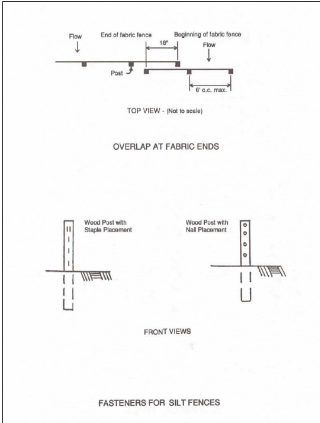
Figure SB-4 Silt Fence Installation Details
