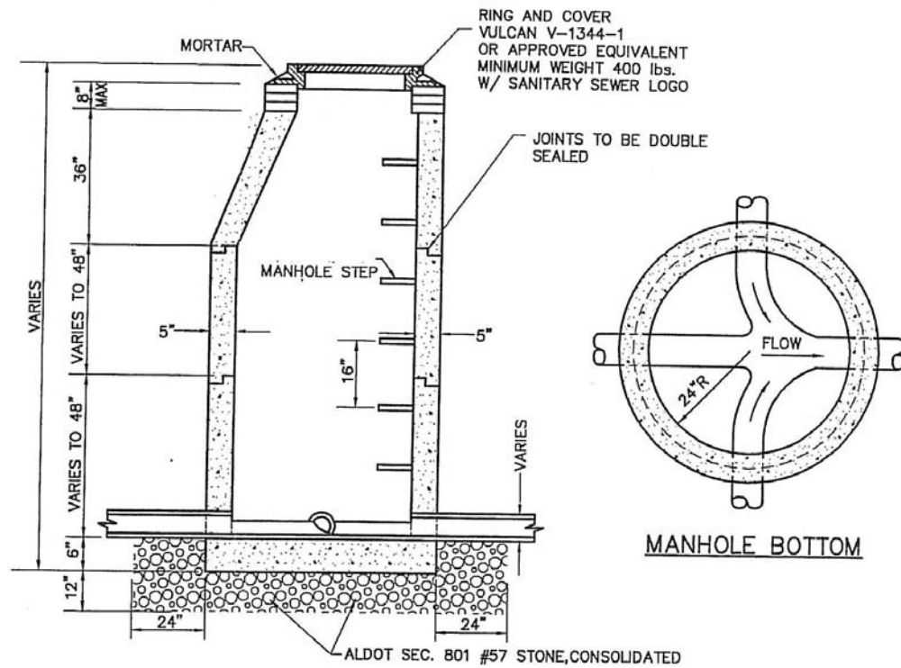
PRECAST ECCENTRIC CONE MANHOLE SECTION
