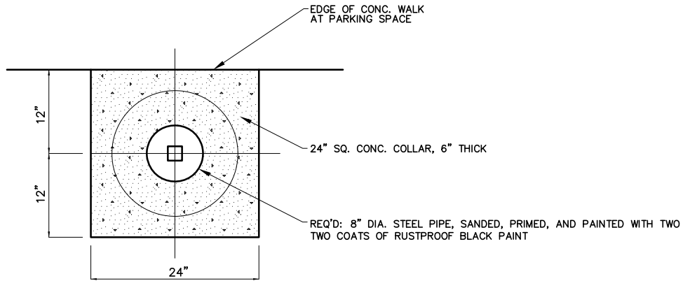
(COLLAR PLAN)
