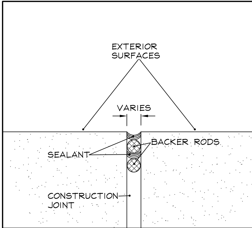
STANDARD DOUBLE SEALANT SECTION SCALE: 1"=1"
