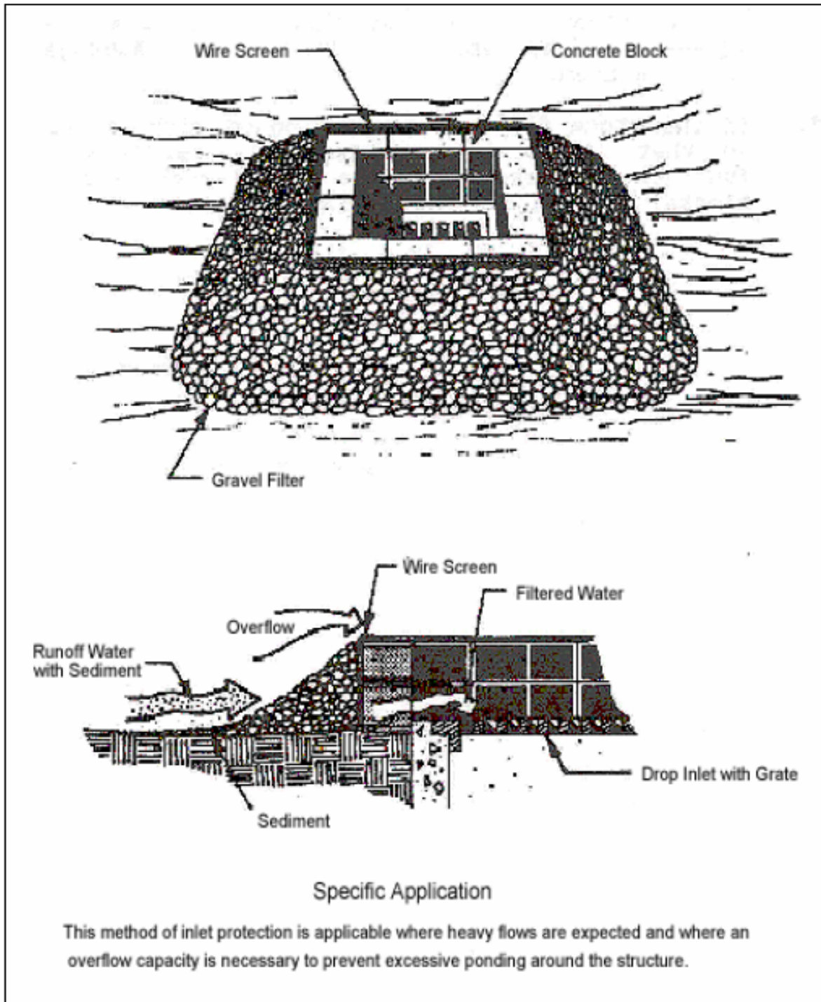
Figure BIP-1 Typical Details of Block and Gravel Inlet Protection
